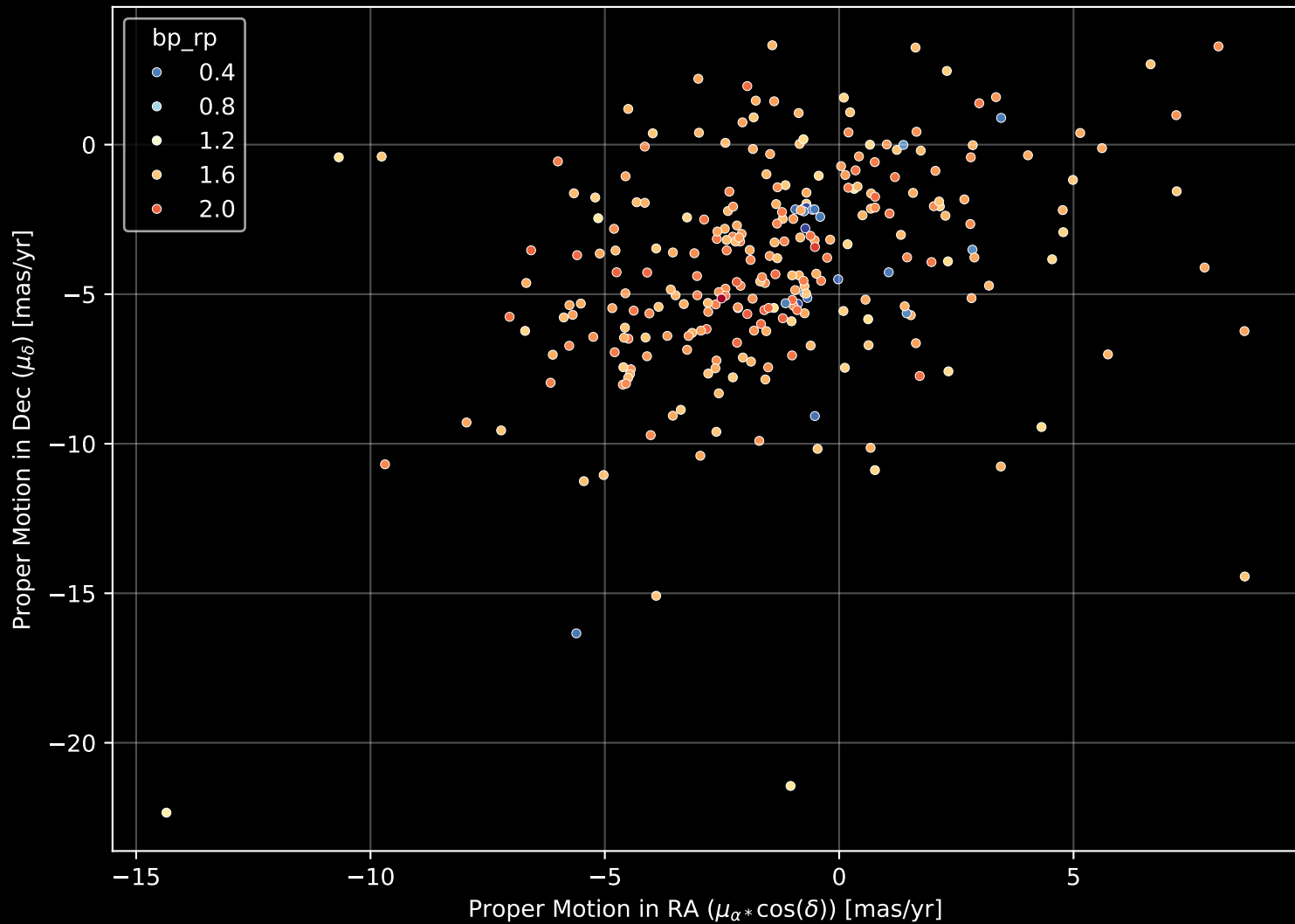
APOGEE DR17 Field: [COROTC] Proper Motion Diagram (n= 273)
