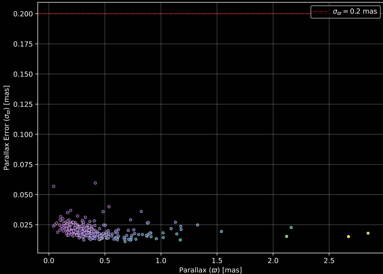
APOGEE DR17 Field: [COROTC] Parallax Quality (n= 273)
