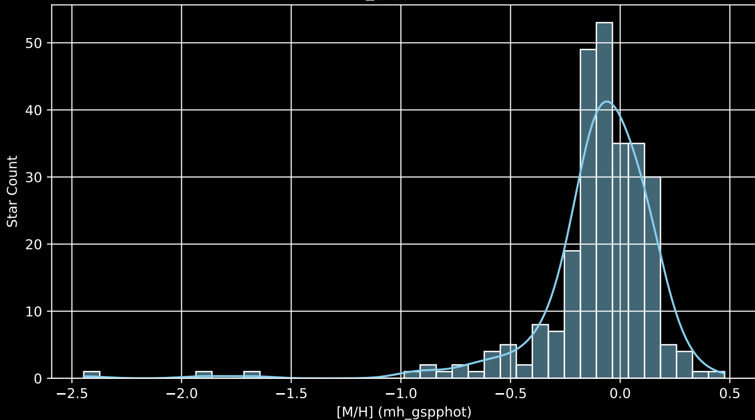
APOGEE DR17 Field: [COROTC [M/H] (mh_gspphot) (n= 268)
