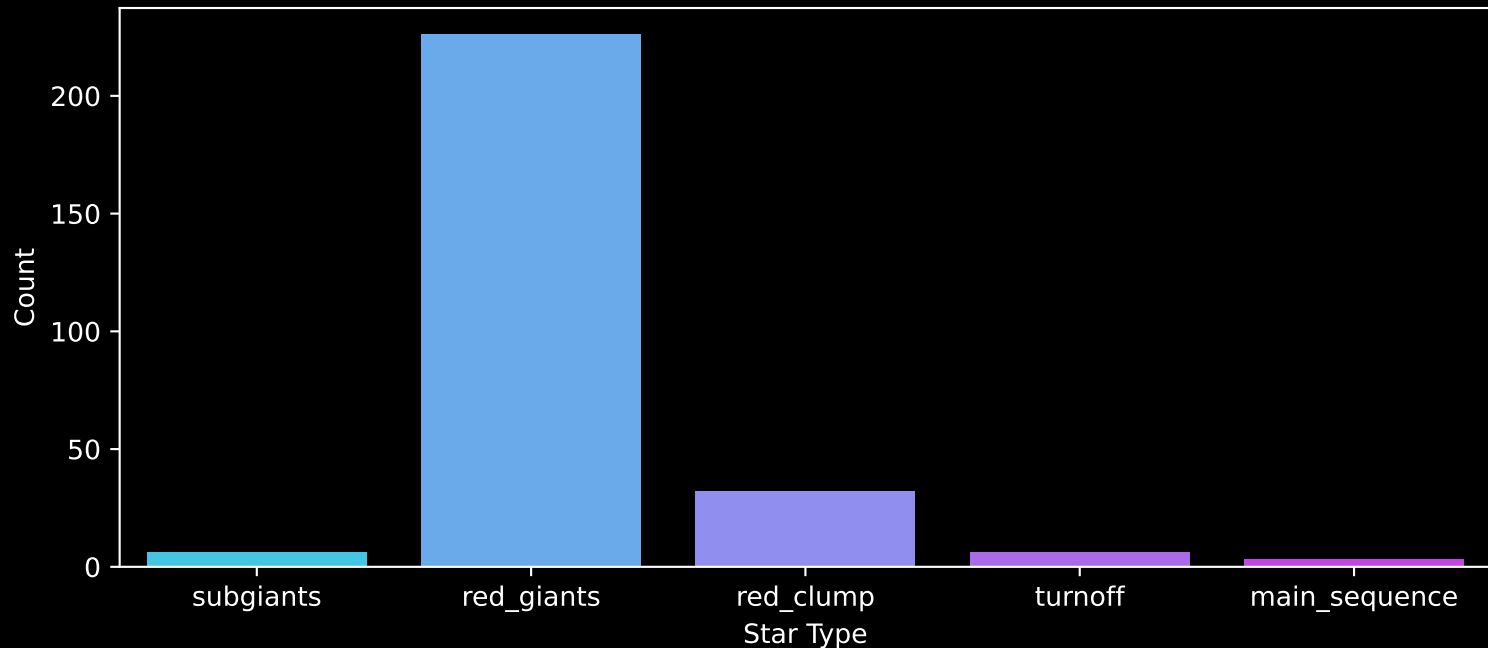
APOGEE DR17 Field: [COROTC] Count plot of Star Type
