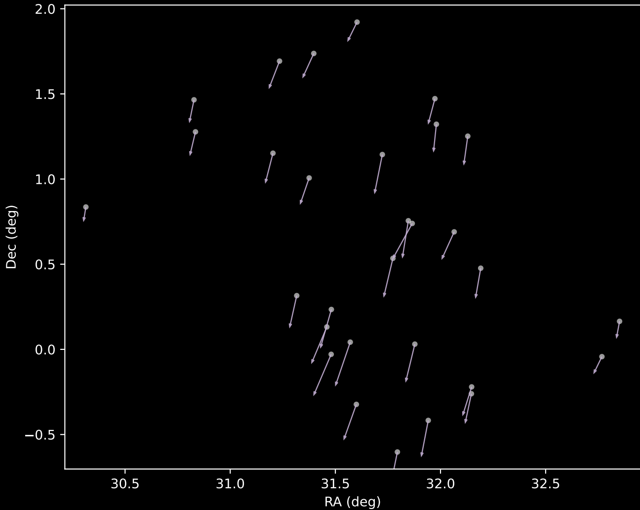
APOGEE DR17 Cluster 9 Proper Motion Vectors (n=30)
