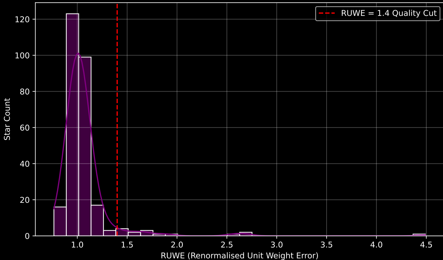
GAPOGEE DR17 Field [COROTC] RUWE Distribution (n= 273)
