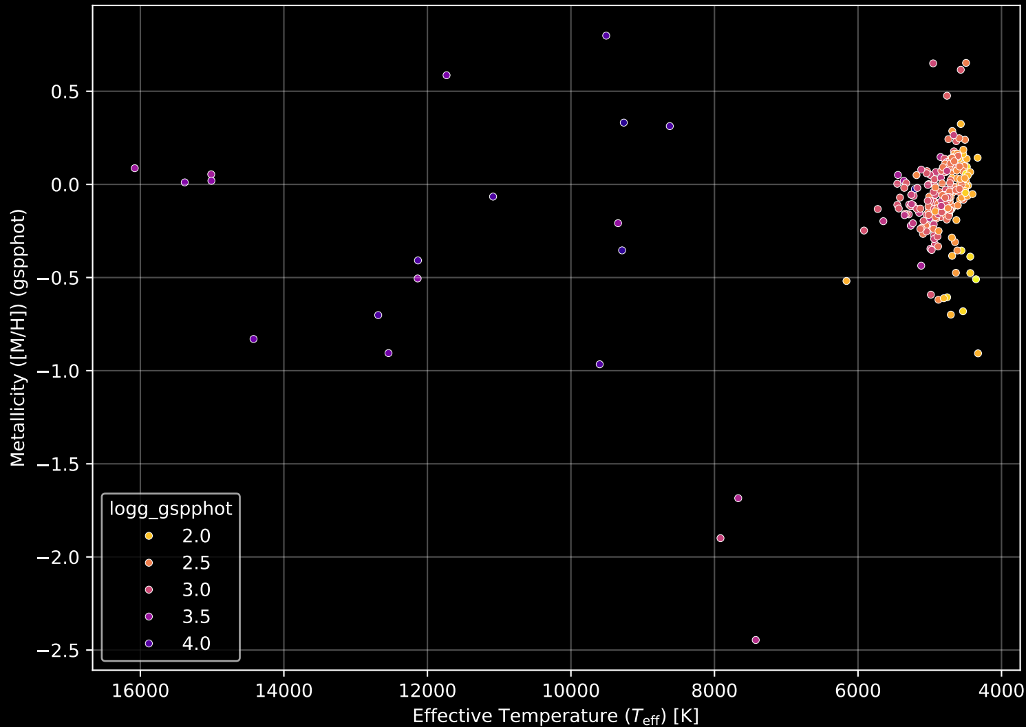
APOGEE DR17 Field: [COROTC] Stellar Population Parameters (n= 273)
