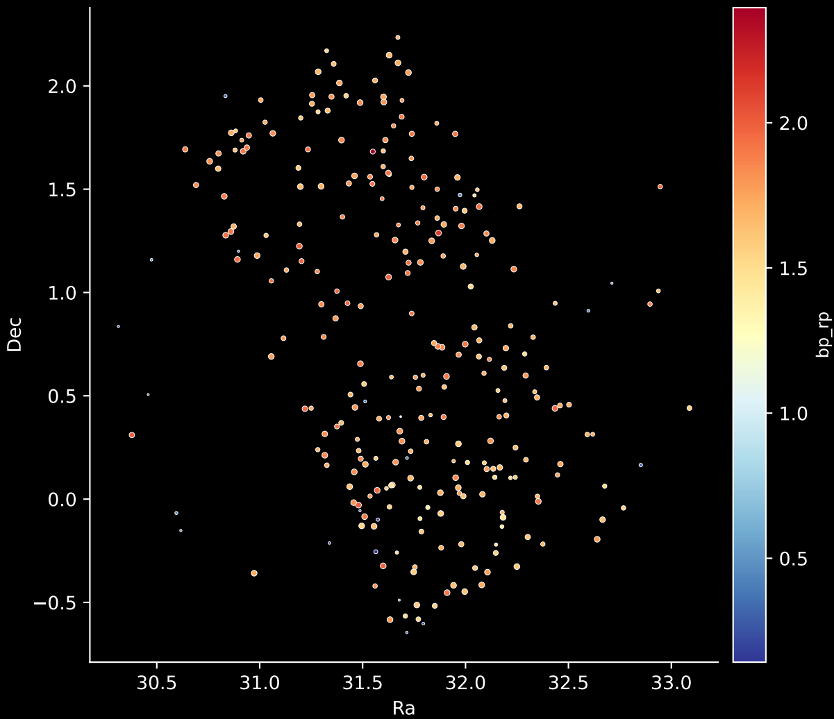
APOGEE DR17 Field: [COROTC] Stars: 273
